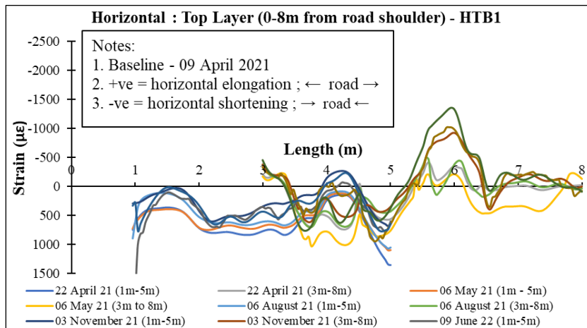
Figure 8. Strain Against Length for HTB1
